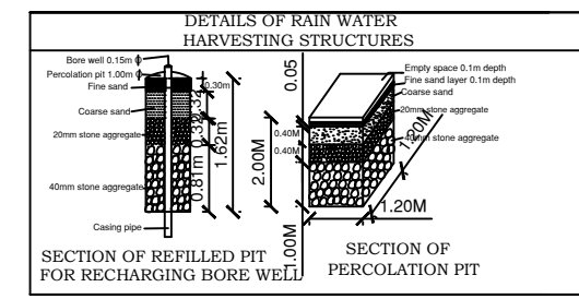
DETAILS OF RAIN WATER HARVESTING STRUCTURES
